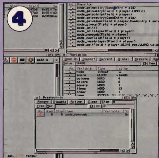
4. Breakpoints are another vital debugging feature as they allow you to pause the running program at a given point and then check the state of it. Here we've paused the program as a particular function is called.
